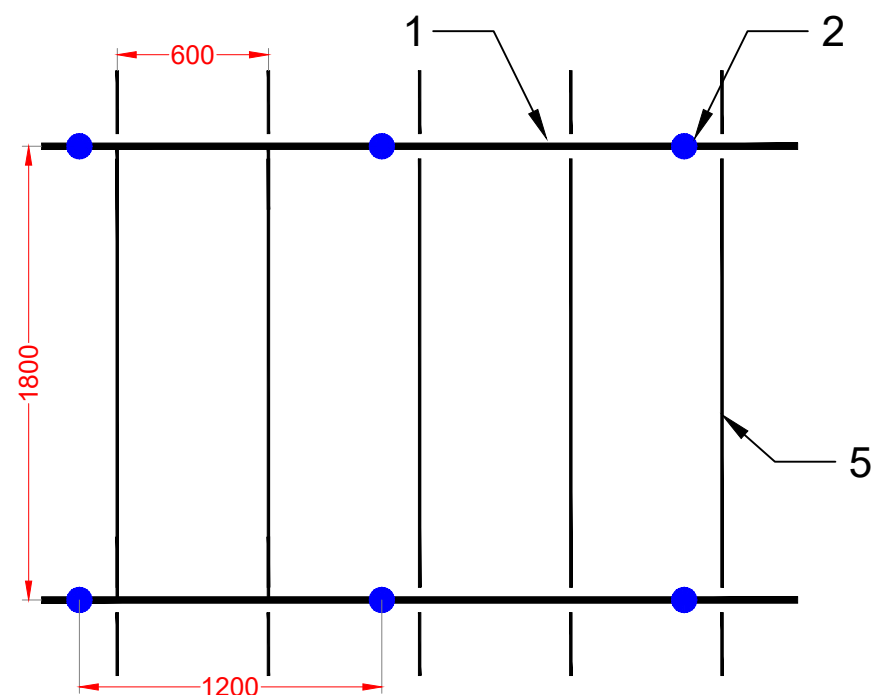
Layout 3: 1800 x 600mm modules
