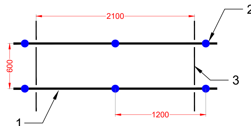
Layout 5: 2100 x 600mm modules
