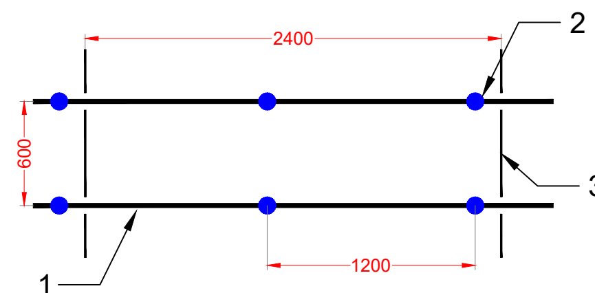
Layout 6: 2400 x 600mm modules
