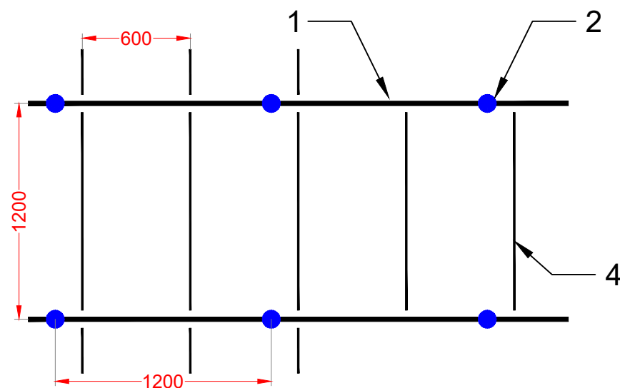
Layout 2: 1200 x 600mm modules
