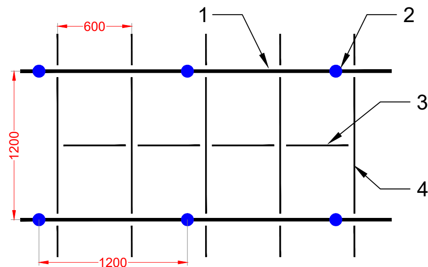
Layout 1: 600 x 600mm modules
