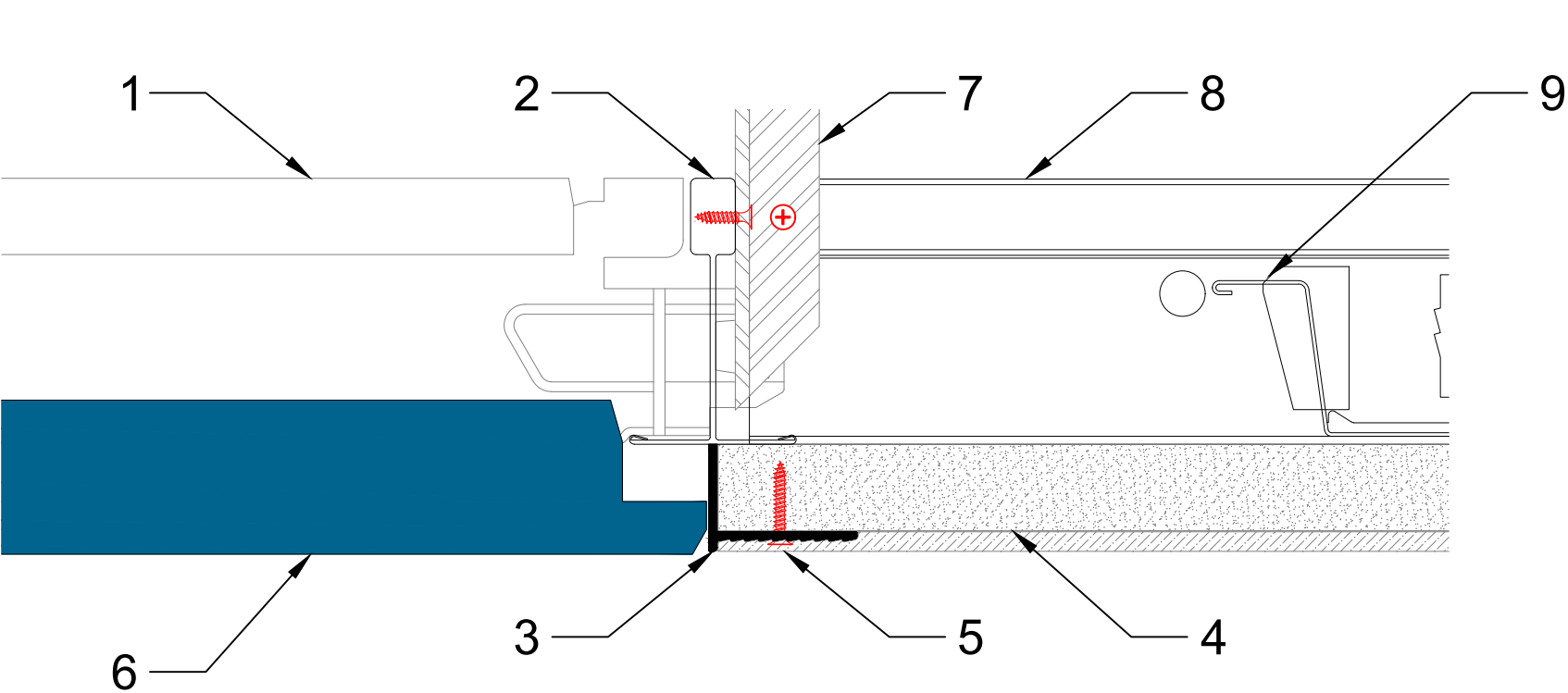
Section B - B: (Unsupported Edge)
