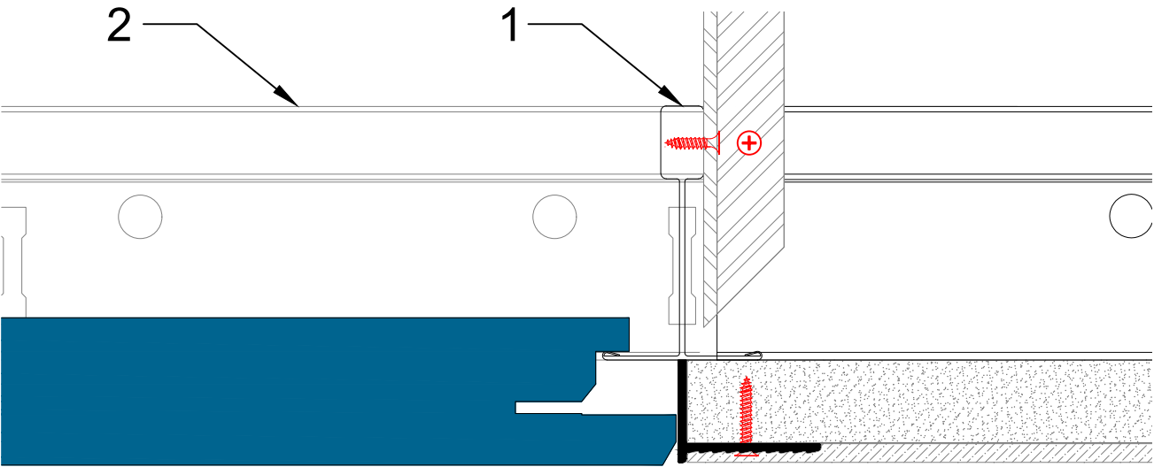
Section A - A: (Supported Edge)
