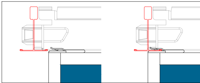
Clips on top of baffles allow connection to T24 grid components
